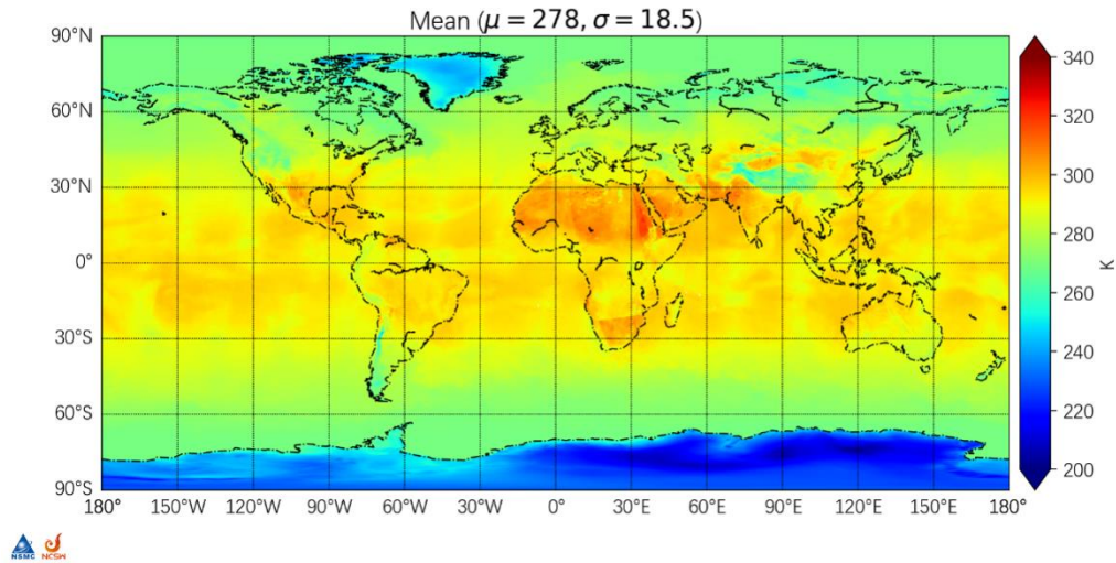
Geographic Statistics of FY3H MERSI 2024-05-08 RTTOV_ERA5137 04_8.55 \mu m
