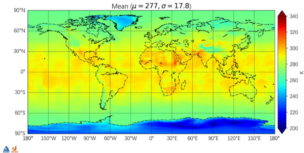
Geographic Statistics of FY3H MERSI 2024-05-08 RTTOV_ERA5137 03_7.20 \mu m
