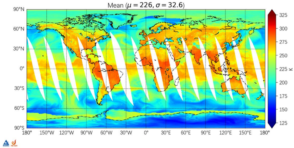
Geographic Statistics of FY3H MWRI 2024-05-13 Sounding_SIM_137 19_118.7503±3.2GHz
